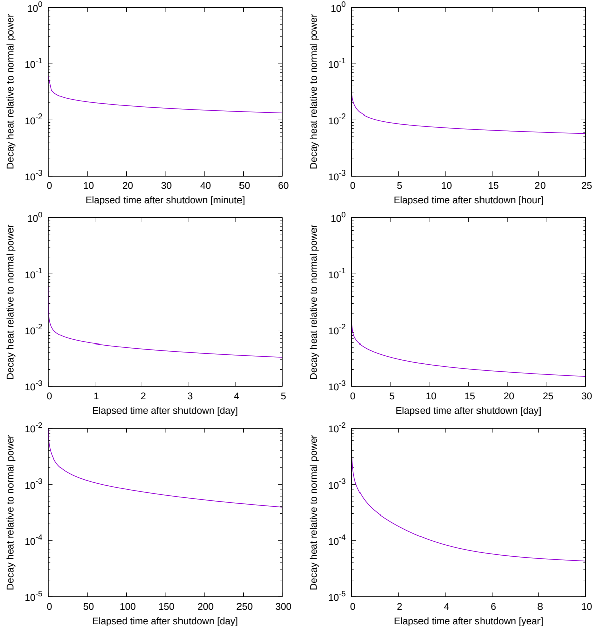
Fig. 1: Decay heat relative to normal power
