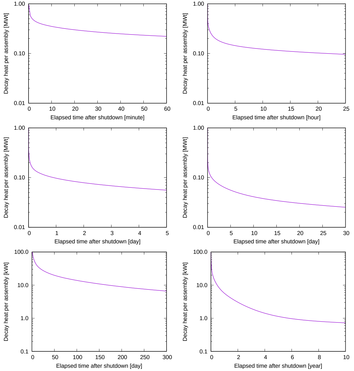
Fig. 2: Decay heat per one fuel assembly
